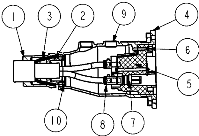
Fig 1a TYPICAL ARMoured GLAND ARRANGEMENT
